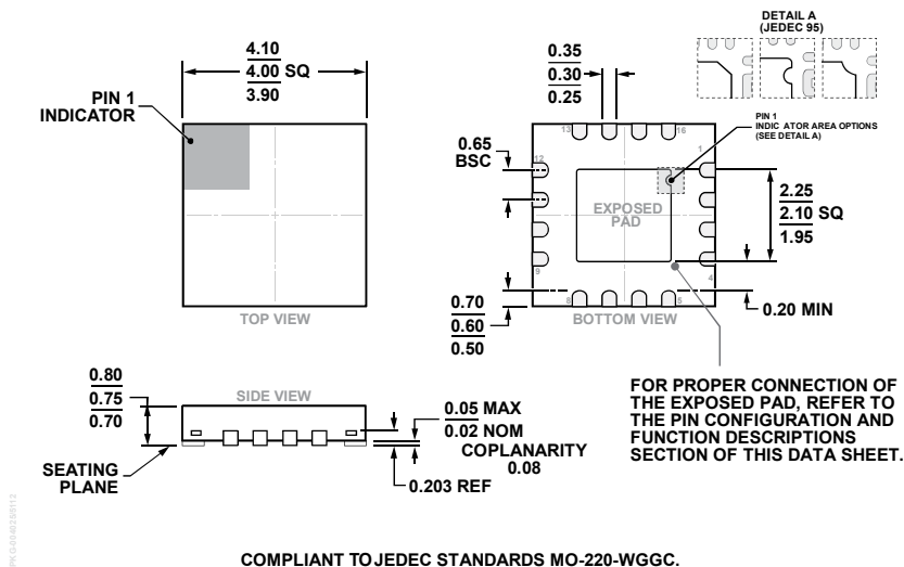
Figure 57. 16-Lead Lead Frame Chip Scale Package [LFCSP] 4 mm × 4 mm Body and 0.75mm Package Height (CP-16-23)
