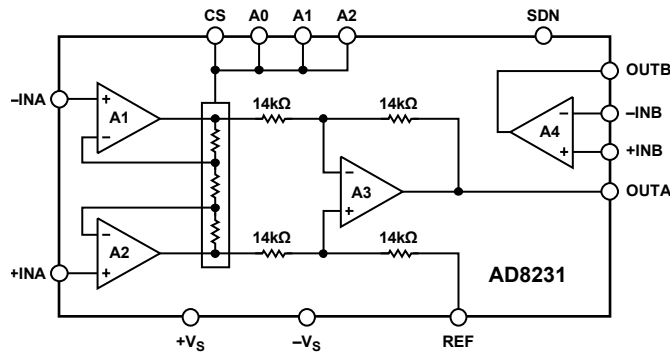
Figure 49. Simplified Schematic
