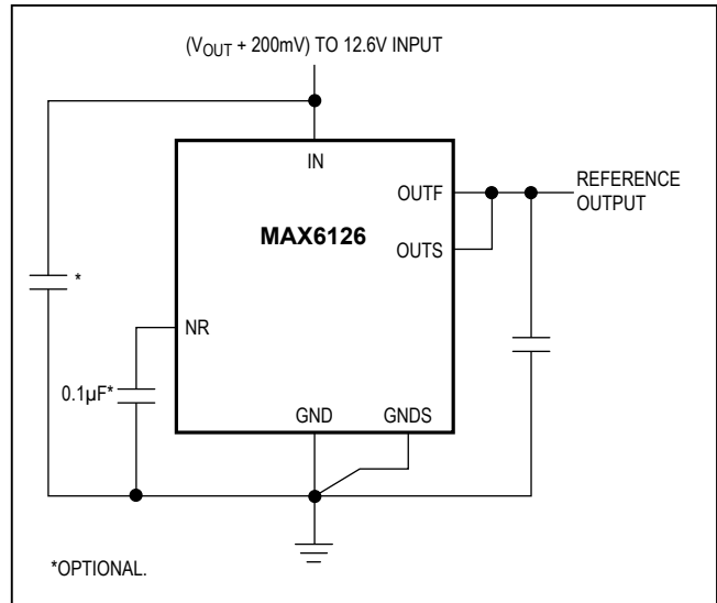
Figure 1. Noise-Reduction Capacitor
