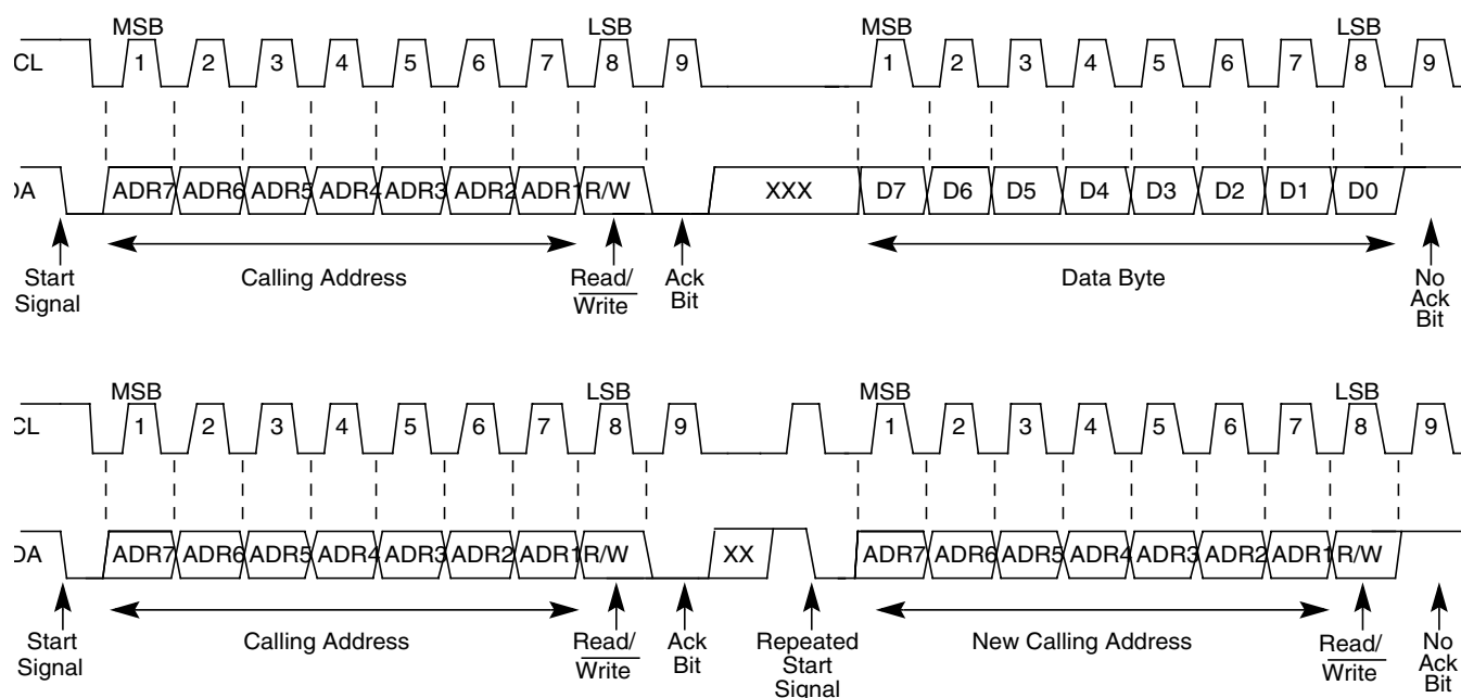
Figure 15-10. IIC-Bus Transmission Signals
