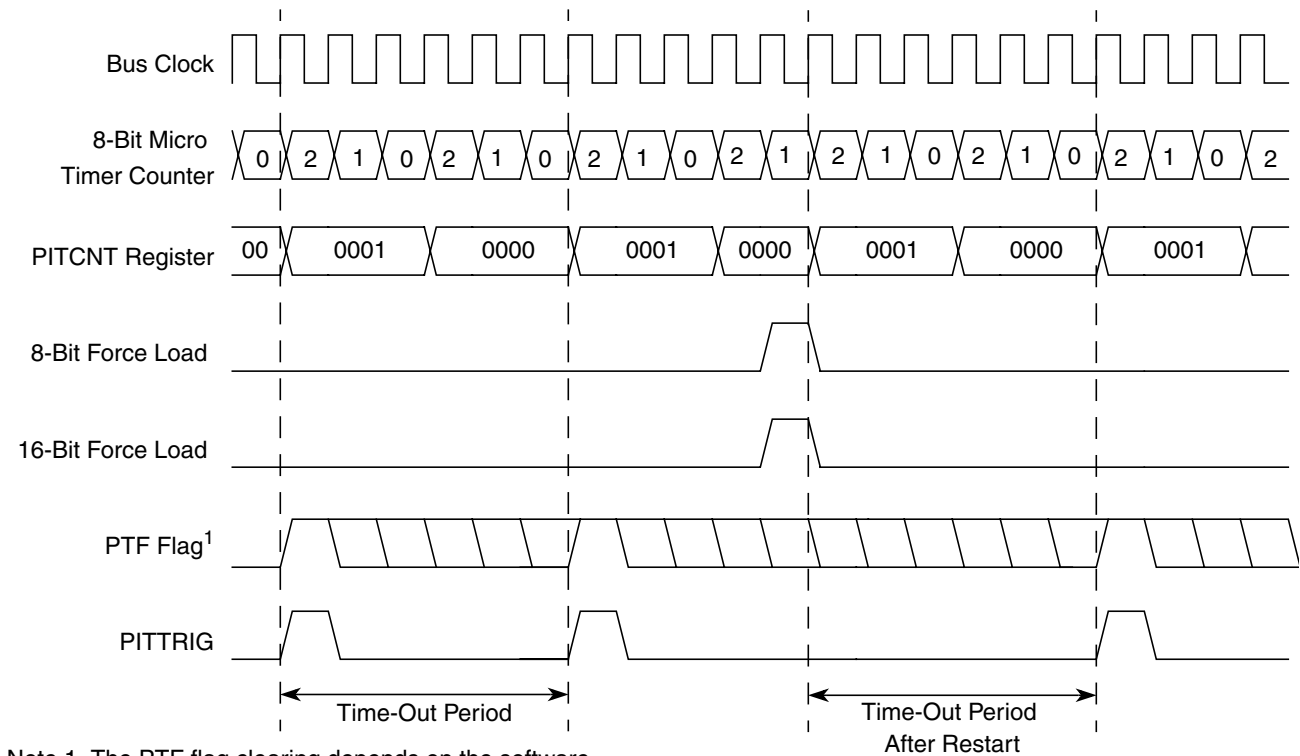
Figure 18-20. PIT Trigger and Flag Signal Timing
