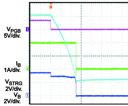
VSTRG Release IB=2A, CSTRG=1000 \mu F
