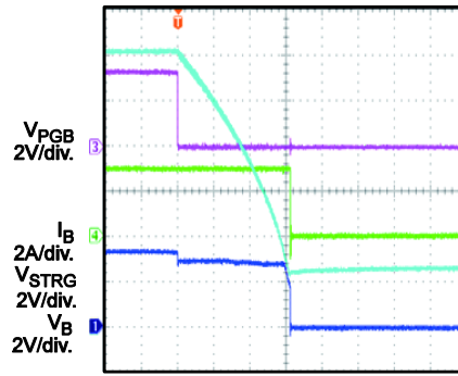
VSTRG Release IB=3A, CSTRG=1000 \mu F
