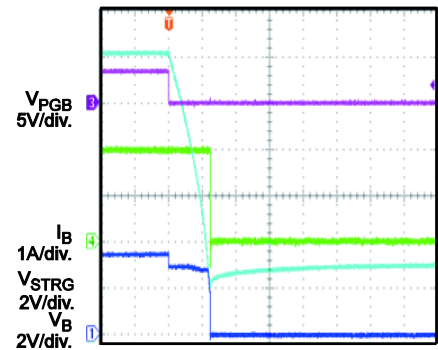
VSTRG Release IB=2A, CSTRG=470 \mu F
