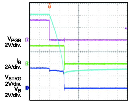
VSTRG Release IB=3A, CSTRG=470 \mu F
