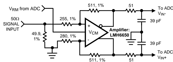
Figure 38. Optional Amplifier Differential Drive Circuit
