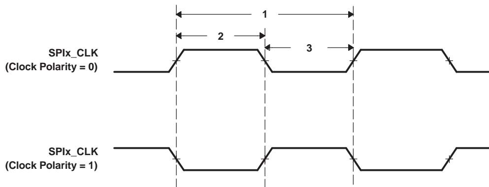
Figure 6-62. SPI_CLK Timing
