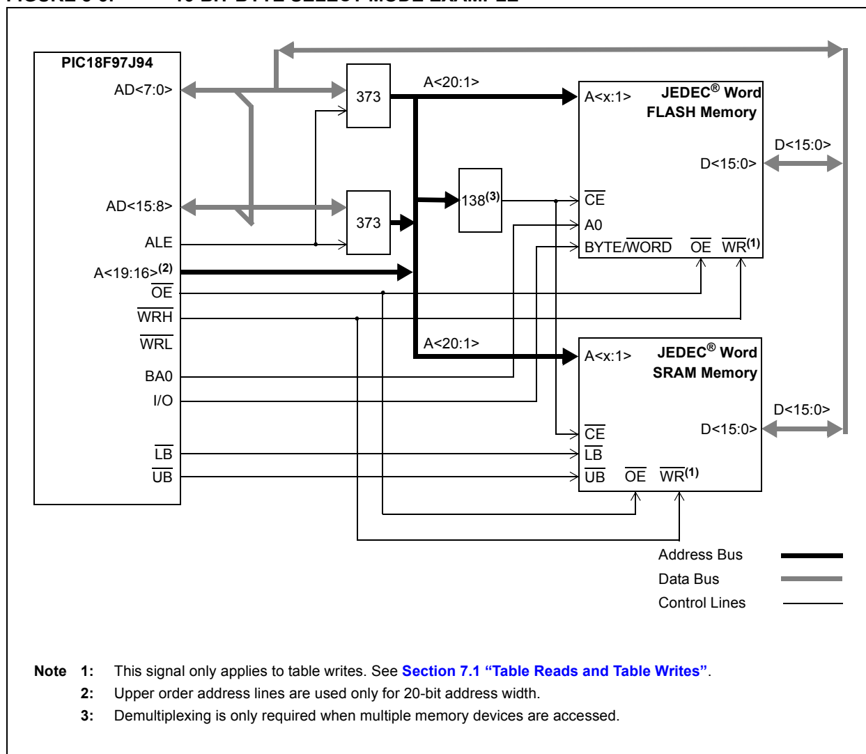
FIGURE 8-3: 16-BIT BYTE SELECT MODE EXAMPLE
