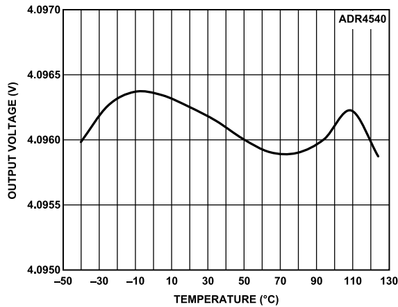
Figure 65. ADR4540 B Grade Output Voltage vs. Temperature
