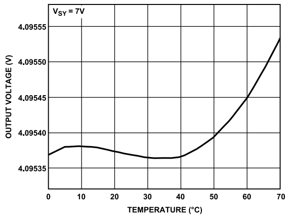
Figure 66. ADR4540 C Grade Output Voltage vs. Temperature
