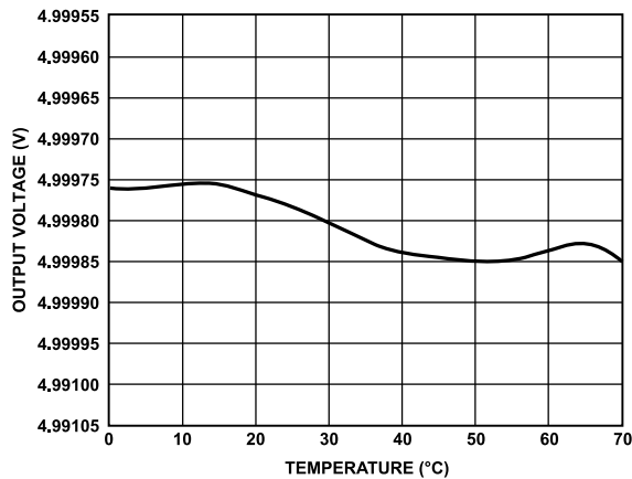
Figure 67. ADR4540 D Grade Output Voltage vs. Temperature
