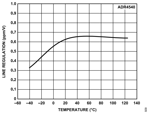
Figure 72. ADR4540 Line Regulation vs. Temperature
