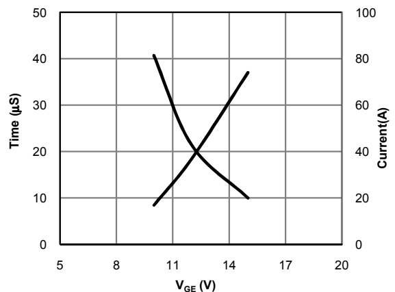
Fig 6: V_{GE} vs. Short Circuit Time ( V_{CE}=400V, T_C=25^\circ\text{C} )
