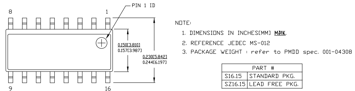
Figure 14. 16-pin SOIC (150 Mils) S16.15/SZ16.15 Package Outline, 51-85068
