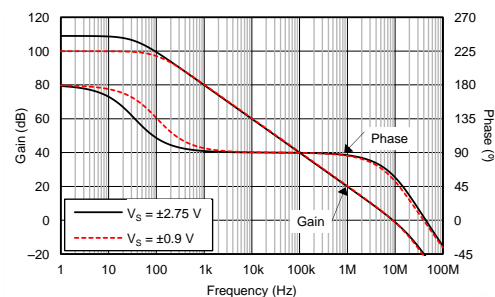
Low-Supply Current (400 \mu\text{A}/\text{ch} ) for 10-MHz Bandwidth
