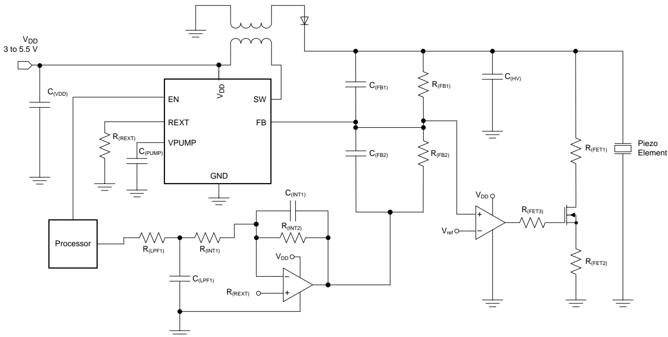
Figure 37. Flyback Circuit
