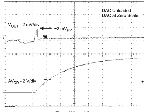
POWER-ON GLITCH RESET TO ZERO SCALE
