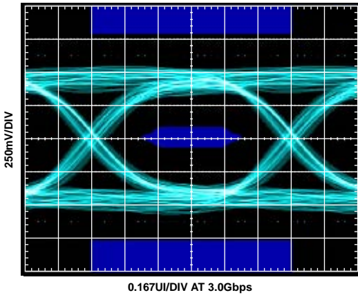
Figure 15. Tx Eye Diagram at TP2, PE = 0 dB, Data Rate = 3.0 Gbps
