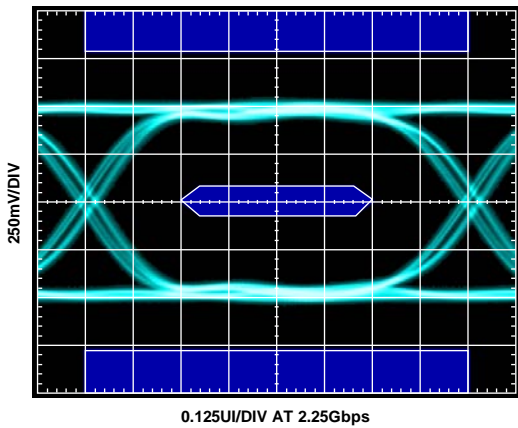
Figure 14. Tx Eye Diagram at TP2, PE = 0 dB, Data Rate = 2.25 Gbps
