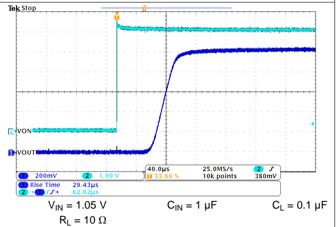
Figure 20. t_R at V_{IN} = 1.05\text{ V}
