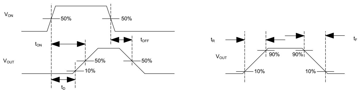
Figure 34. Timing Waveforms
