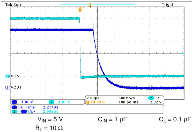
Figure 17. t_F at V_{IN} = 5\text{ V}
