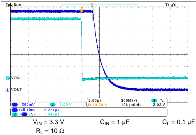
Figure 19. t_F at V_{IN} = 3.3\text{ V}
