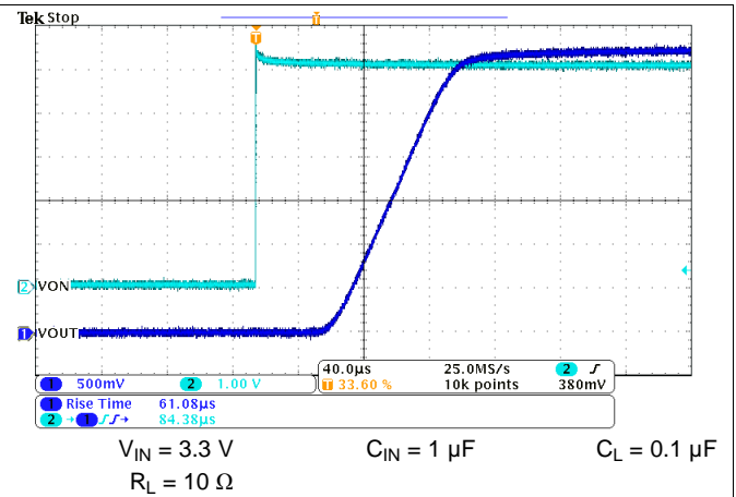
Figure 18. t_R at V_{IN} = 3.3\text{ V}
