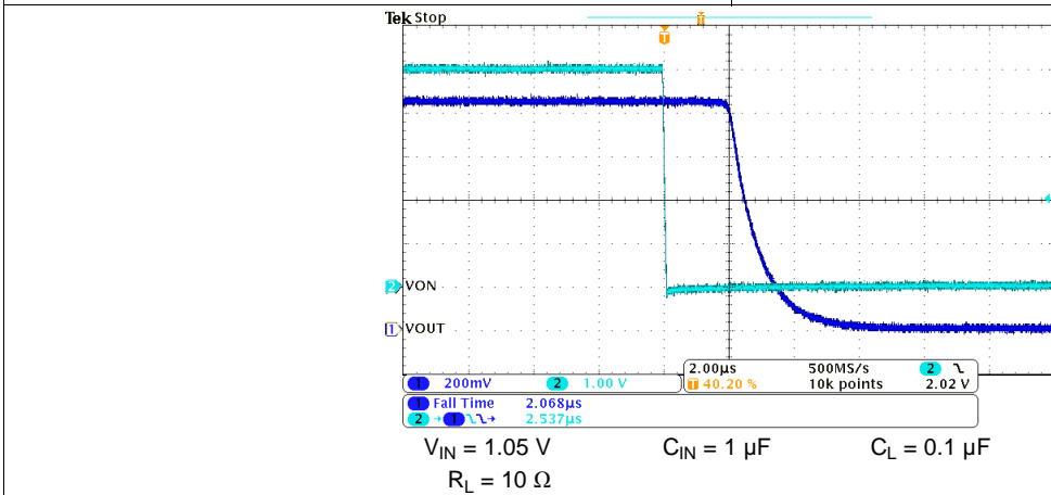
Figure 21. t_F at V_{IN} = 1.05\text{ V}
