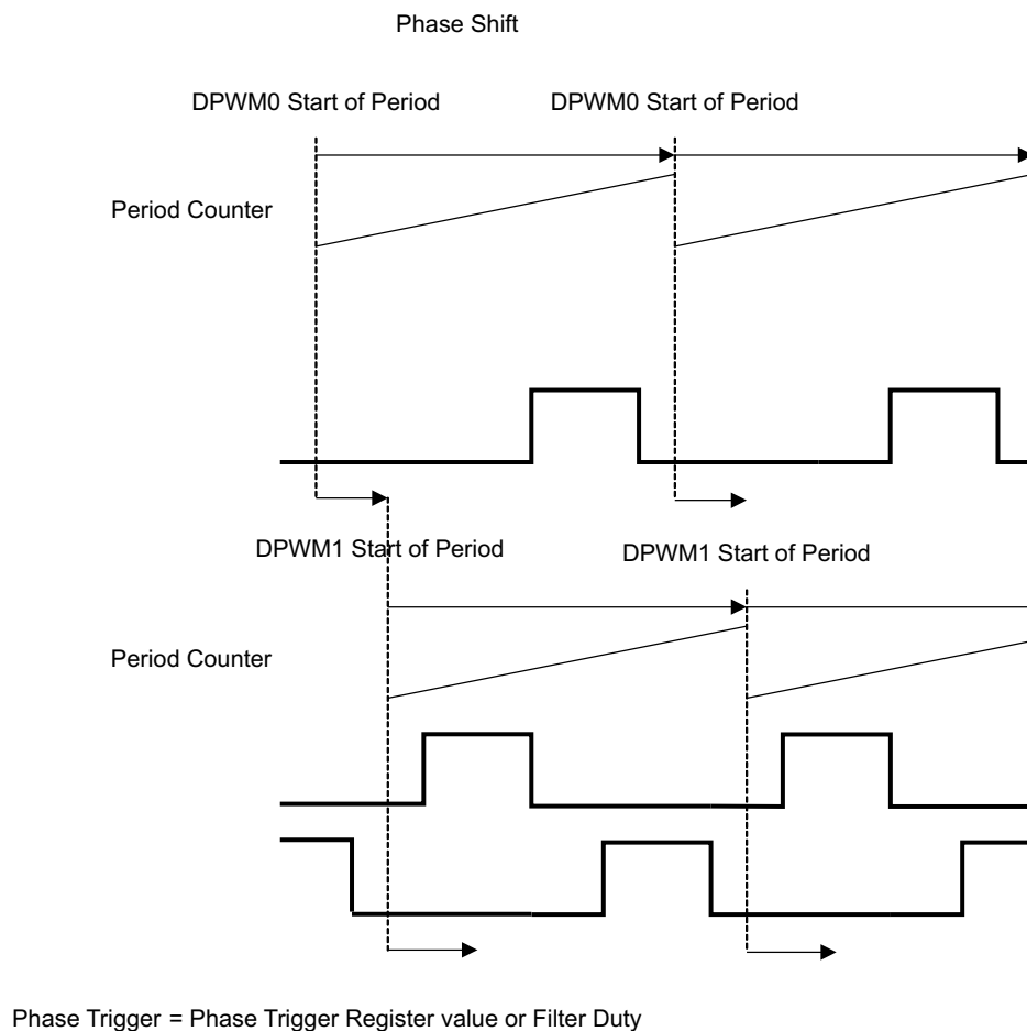
Figure 6-18. Phase Shift
