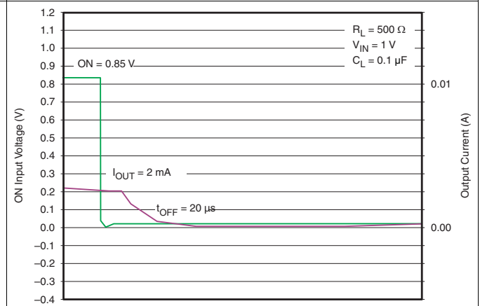
Figure 33. t_{OFF} Response
