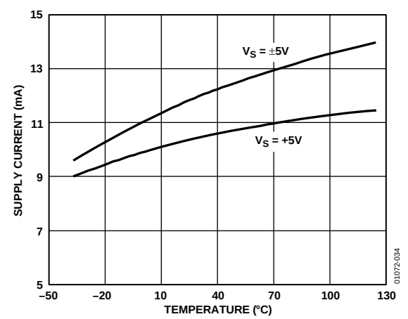
Figure 34. Quiescent Current vs. Temperature
