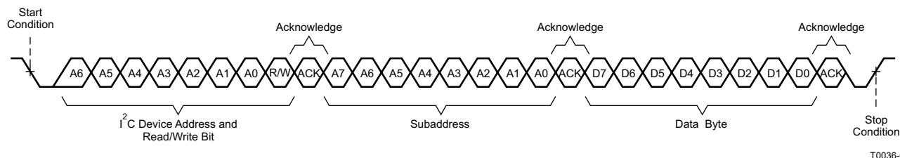
Figure 17. Random Write Transfer
