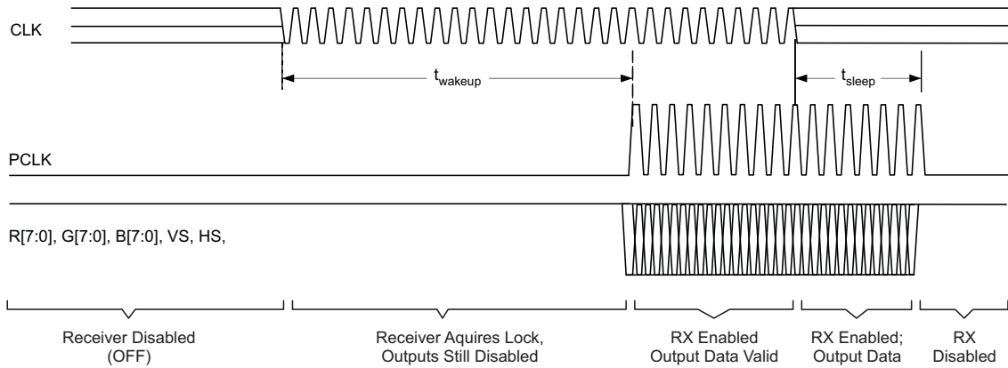
Figure 15. Standby Detection
