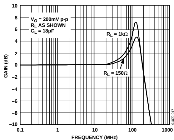
Figure 12. AD8115 Frequency Response vs. Load Impedance
