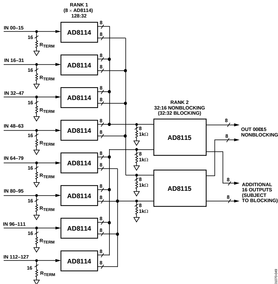
Figure 49. Nonblocking 128 \times 16 Array ( 128 \times 32 Blocking)
