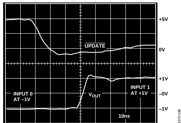
Figure 33. AD8114 Switching Time
