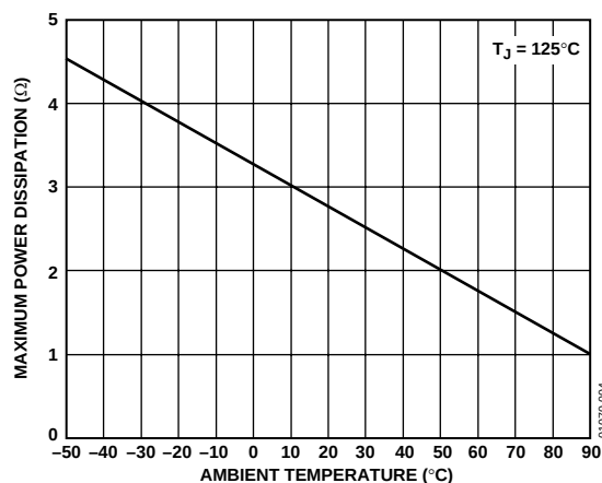
Figure 5. Maximum Power Dissipation vs. Temperature
