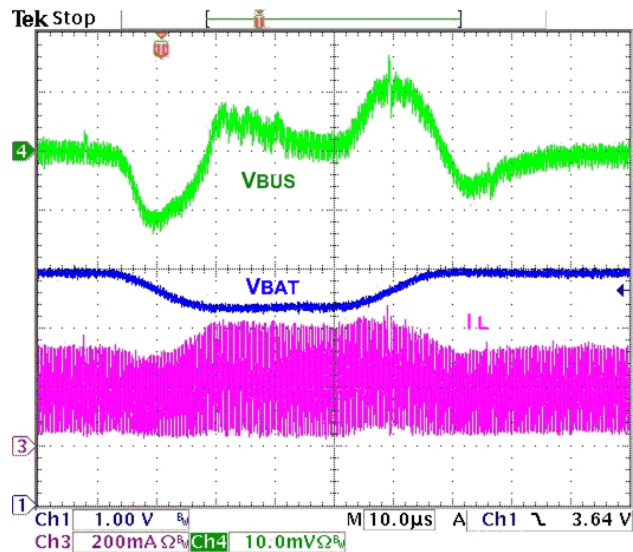
Figure 34. Line Transient, 50 \Omega Load, 3.9-3.3-3.9 V_{BAT} , t_{RISE}/t_{FALL}=10\text{ }\mu\text{s}
