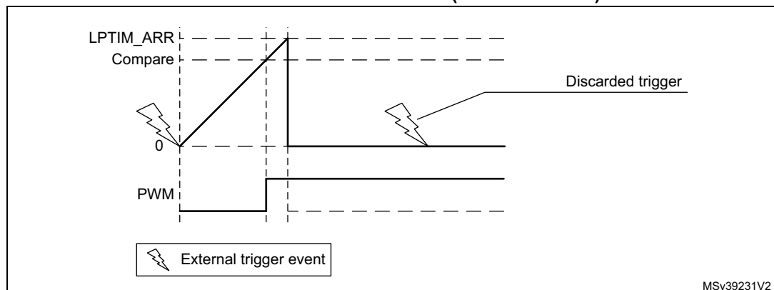
Figure 341. LPTIM output waveform, Single counting mode configuration and Set-once mode activated (WAVE bit is set)
