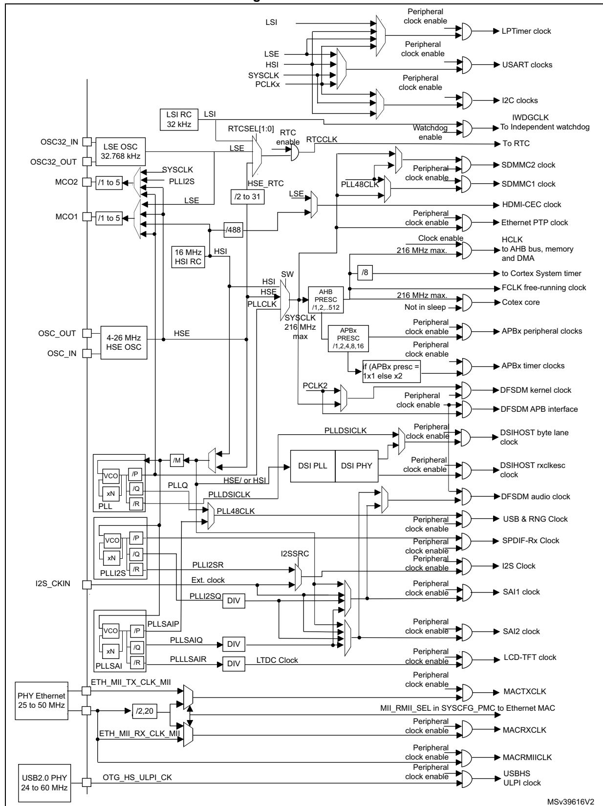
Figure 13. Clock tree
