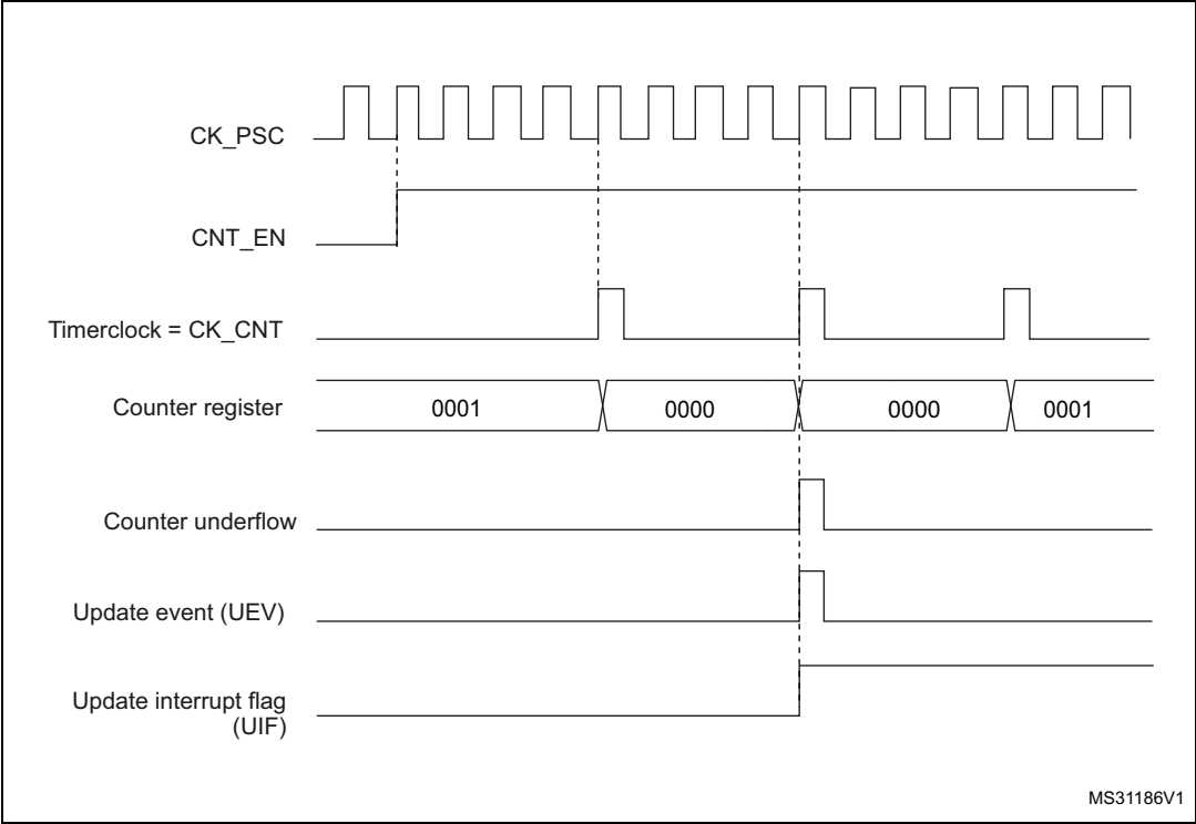
Figure 265. Counter timing diagram, internal clock divided by N
