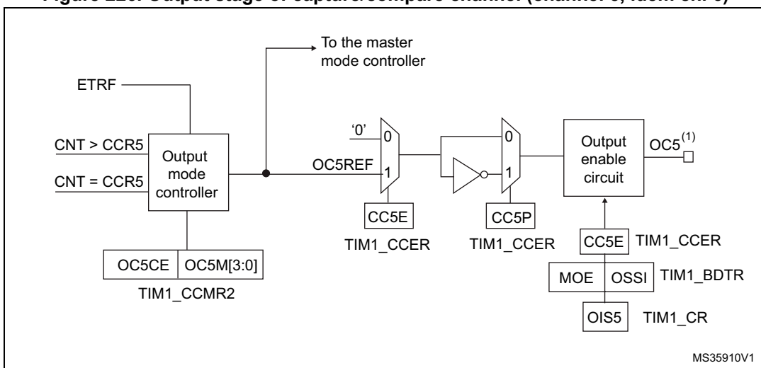
Figure 226. Output stage of capture/compare channel (channel 5, idem ch. 6)
