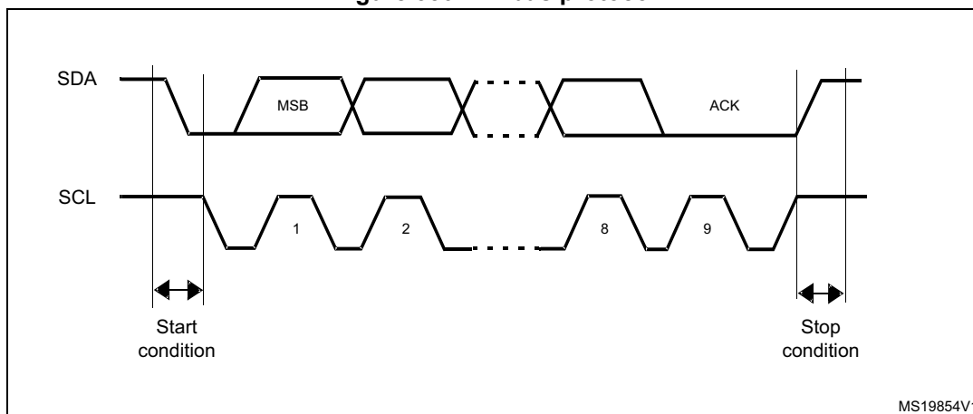
Figure 350. I 2 C bus protocol
