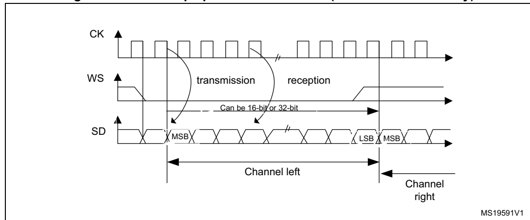
Figure 423. I 2 S Philips protocol waveforms (16/32-bit full accuracy)
