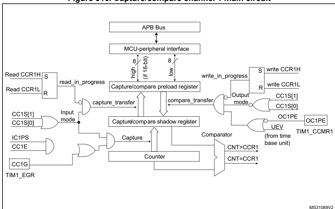
Figure 316. Capture/compare channel 1 main circuit
