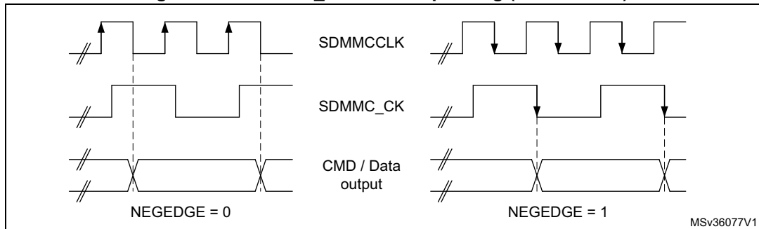
Figure 486. SDMMC_CK clock dephasing (BYPASS = 0)
