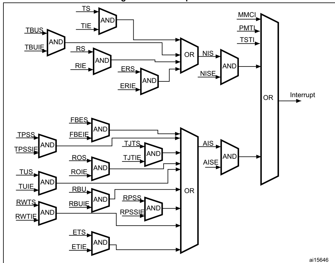
Figure 575. Interrupt scheme
