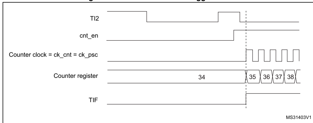
Figure 294. Control circuit in trigger mode
