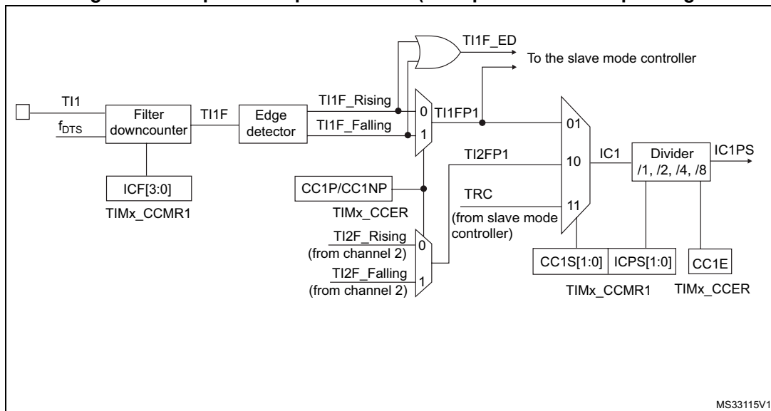
Figure 315. Capture/compare channel (example: channel 1 input stage)
