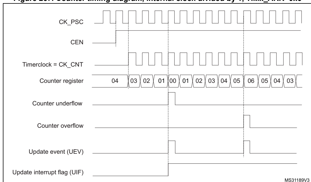
Figure 267. Counter timing diagram, internal clock divided by 1, TIMx_ARR=0x6
