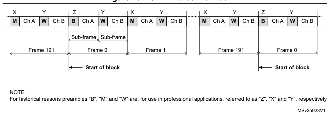
Figure 461. S/PDIF block format
