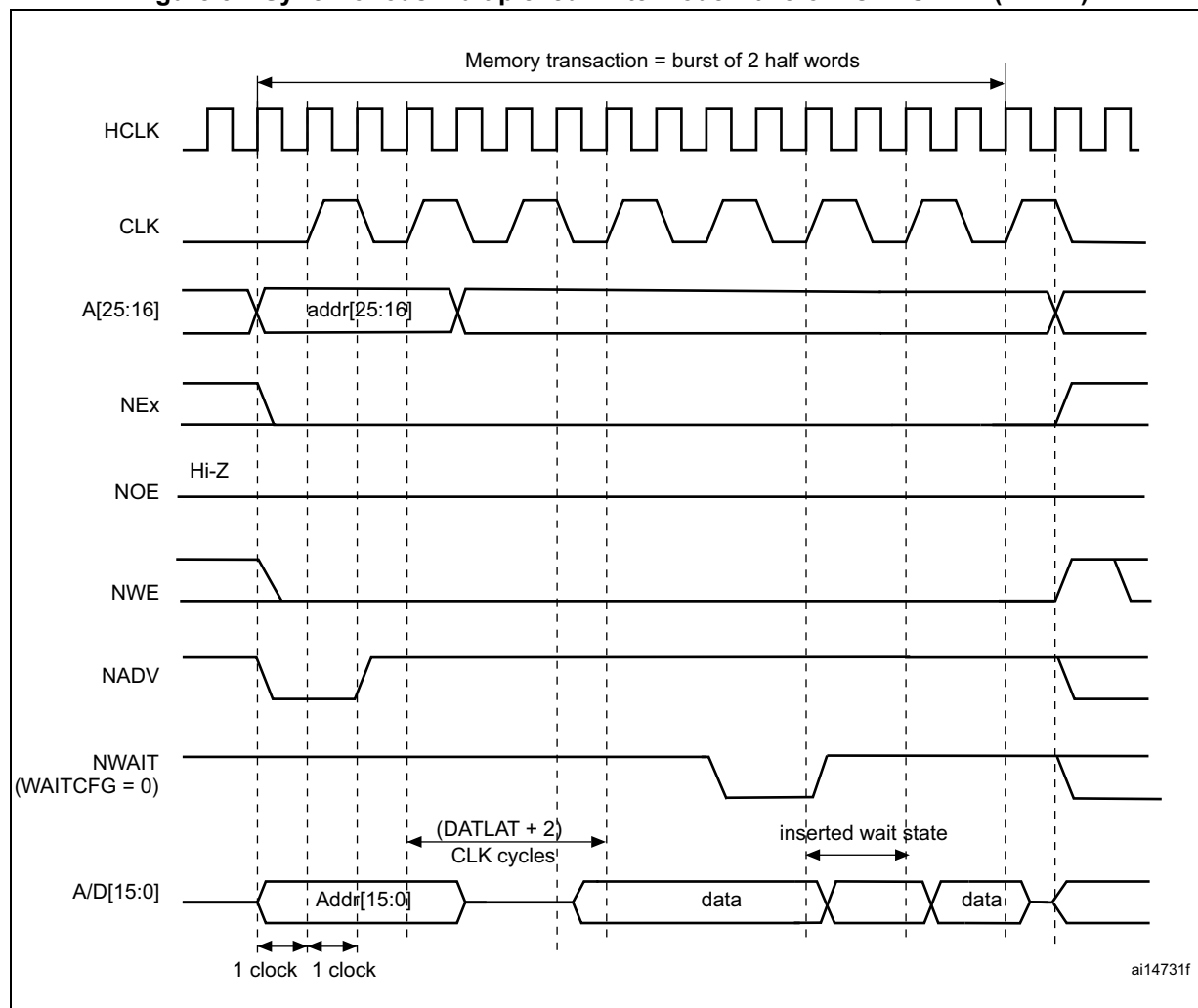
Figure 52. Synchronous multiplexed write mode waveforms - PSRAM (GRAM)
