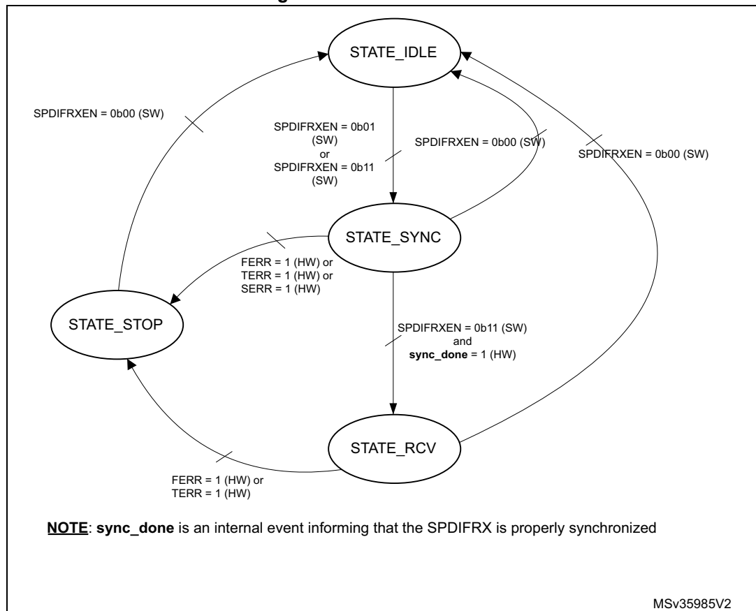
Figure 469. SPDIFRX States
