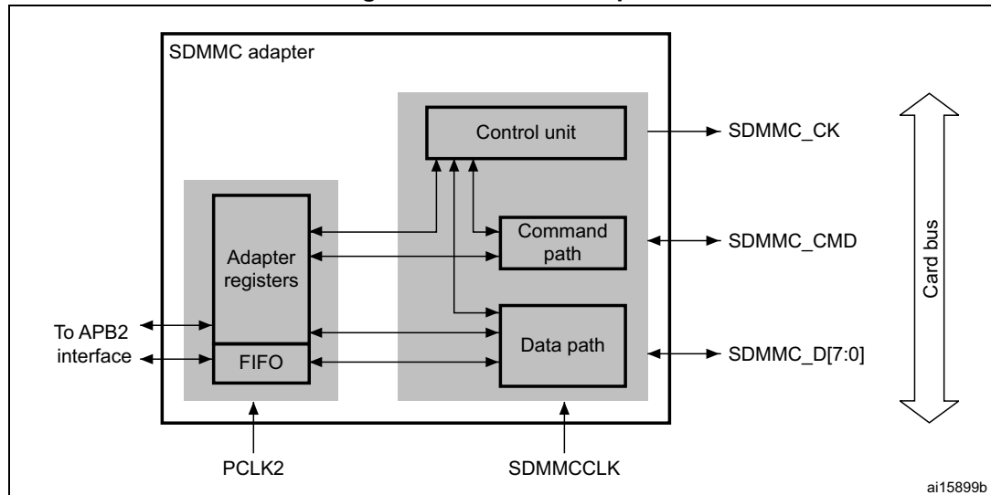
Figure 484. SDMMC adapter
