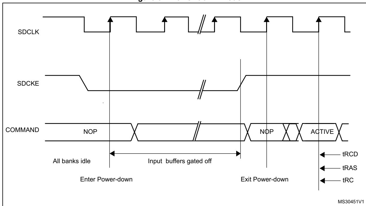
Figure 61. Power-down mode
