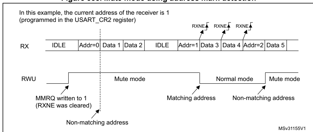
Figure 388. Mute mode using address mark detection
