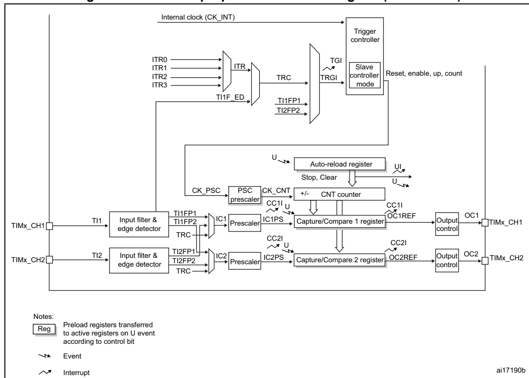
Figure 302. General-purpose timer block diagram (TIM9/TIM12)
