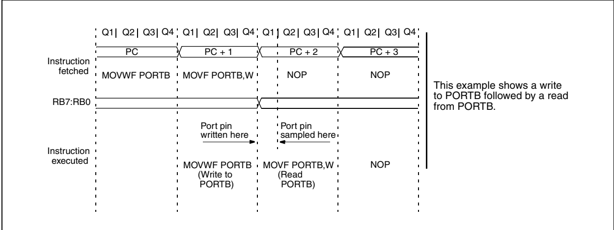
FIGURE 5-5: SUCCESSIVE I/O OPERATION
