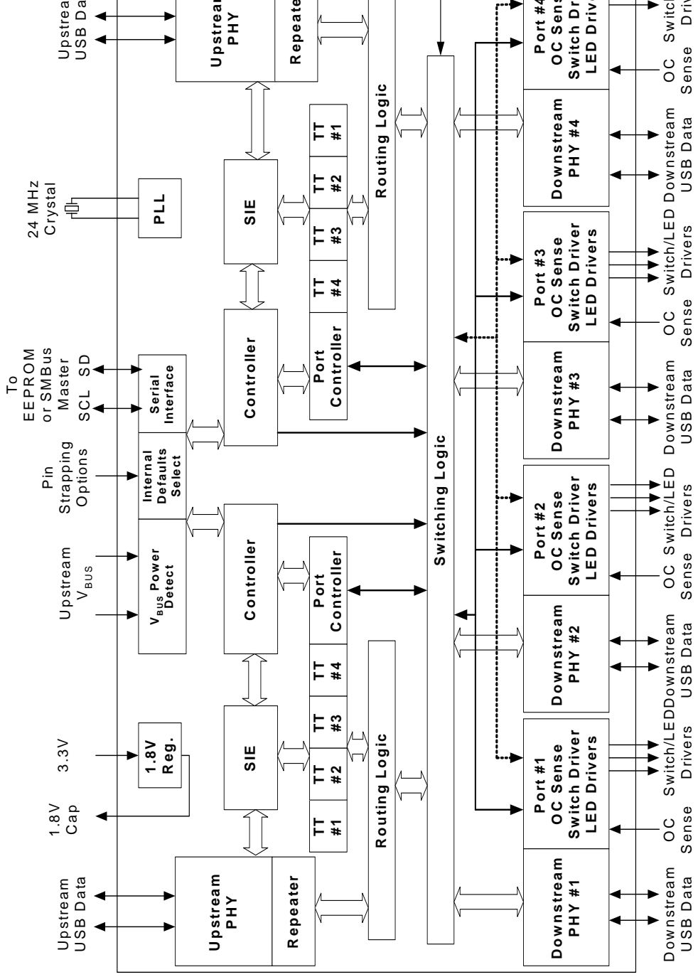
Figure 1 USB2524 Switching Hub Block Diagram
