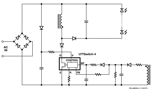
Figure 3d. Typical Buck-Boost Schematic.
