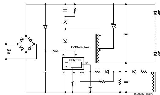
Figure 3c. Typical Tapped-Buck Schematic.
