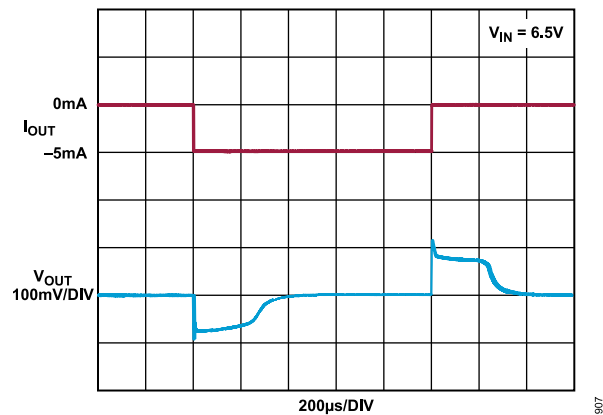
Figure 102. ADR4550 A, B, and C Grades Load Transient Response (Sourcing)
