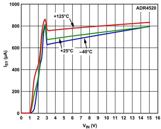
Figure 11. ADR4520 Supply Current ( I_S ) vs. Supply Voltage
