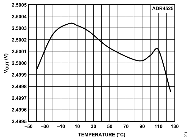
Figure 18. ADR4525 B Grade Output Voltage vs. Temperature
