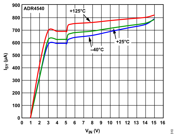
Figure 73. ADR4540 Supply Current vs. Supply Voltage
