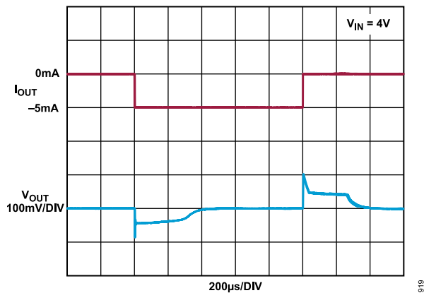
Figure 34. ADR4525 A, B, and C Grades Load Transient Response (Sourcing)
