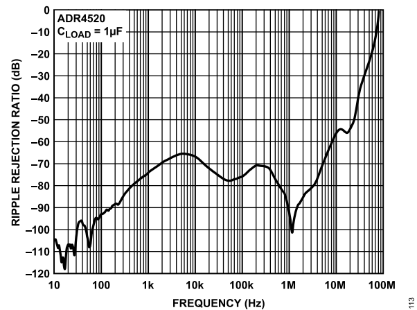
Figure 14. ADR4520 Ripple Rejection Ratio vs. Frequency
