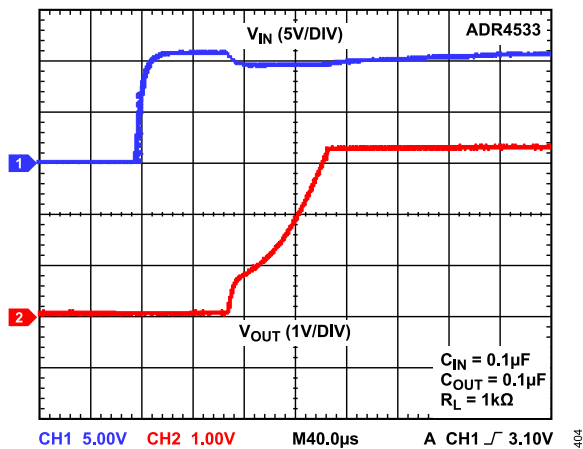
Figure 53. ADR4533 Output Voltage Start-Up Response
