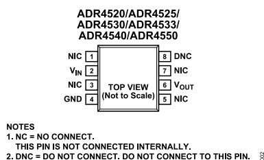
Figure 3. 8-Lead SOIC Pin Configuration
