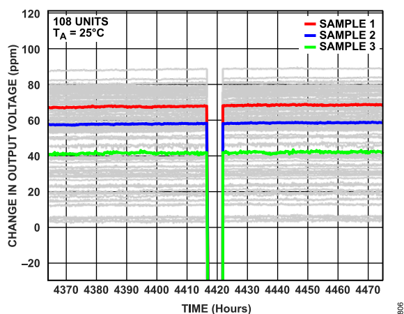
Figure 122. Power Cycle Hysteresis
