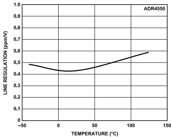
Figure 93. ADR4550 Line Regulation vs. Temperature
