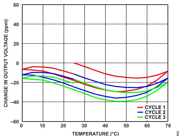
Figure 115. Change in Output Voltage over Three Full Temperature Cycles (0°C to 70°C)
