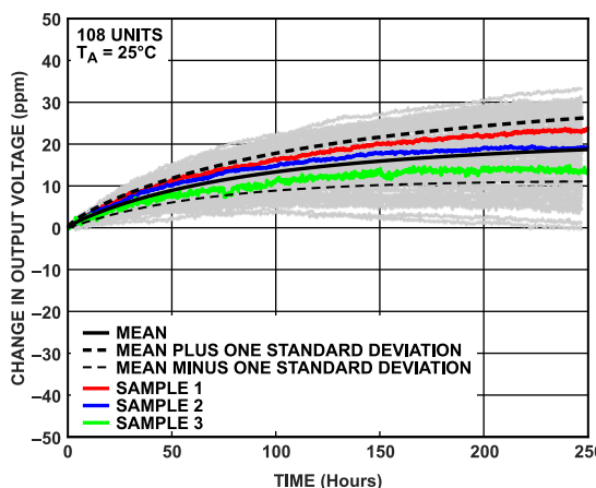
Figure 111. Measured Early Life Drift of the ADR4520/ADR4525/ADR4530/ADR4533/ADR4540/ADR4550
