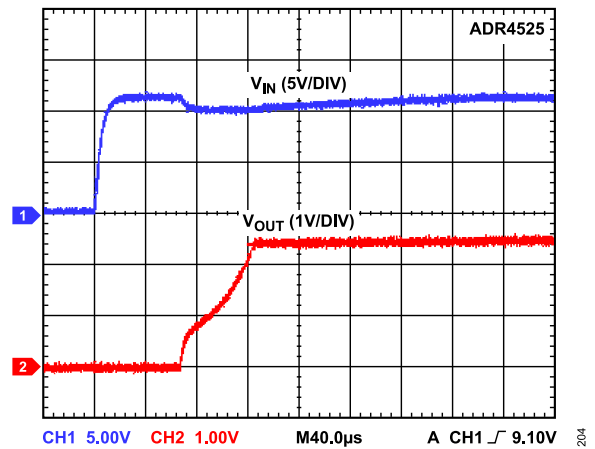
Figure 21. ADR4525 Output Voltage Start-Up Response
