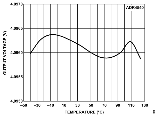
Figure 65. ADR4540 B Grade Output Voltage vs. Temperature
