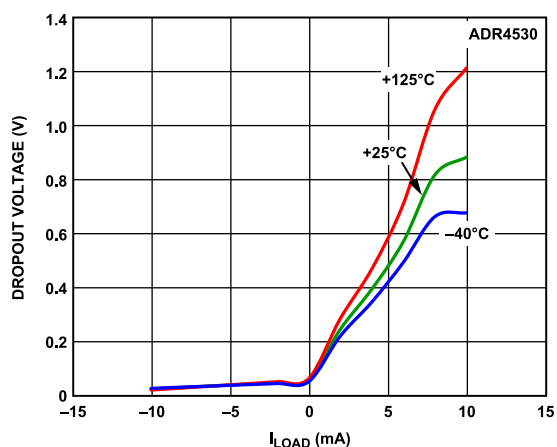
Figure 41. ADR4530 Dropout Voltage vs. Load Current
