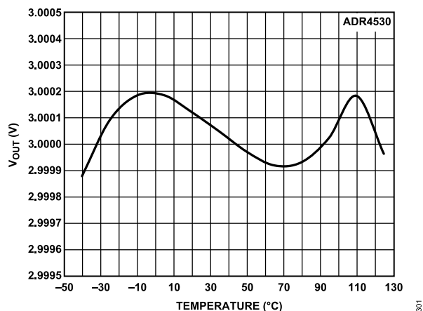
Figure 39. ADR4530 B Grade Output Voltage vs. Temperature
