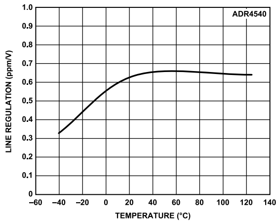
Figure 72. ADR4540 Line Regulation vs. Temperature
