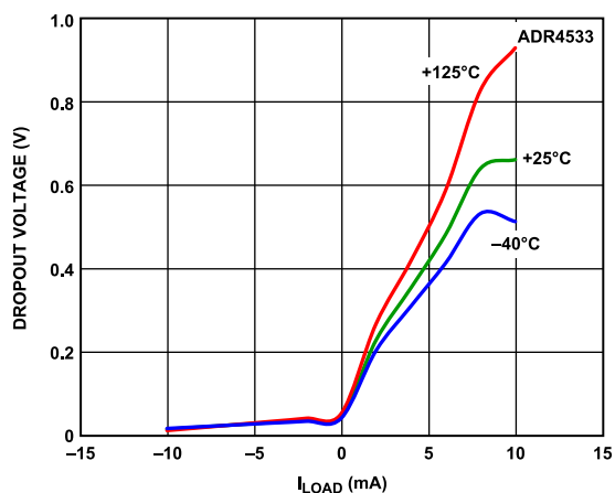
Figure 54. ADR4533 Dropout Voltage vs. Load Current
