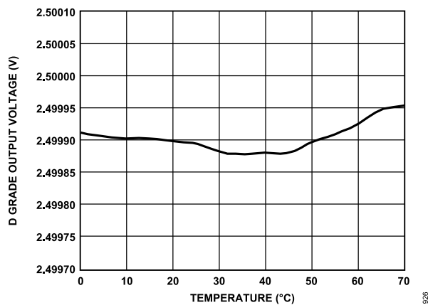
Figure 20. ADR4525 D Grade Output Voltage vs. Temperature
