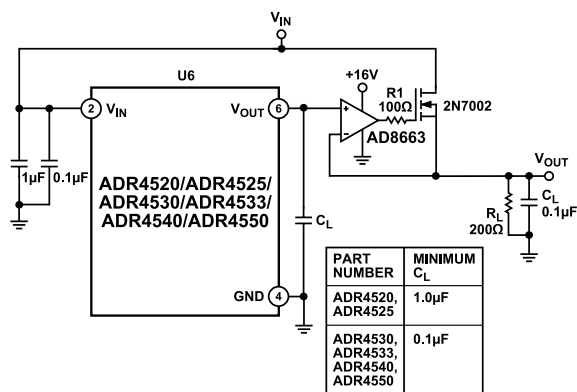
Figure 109. Boosted Output Current Reference
