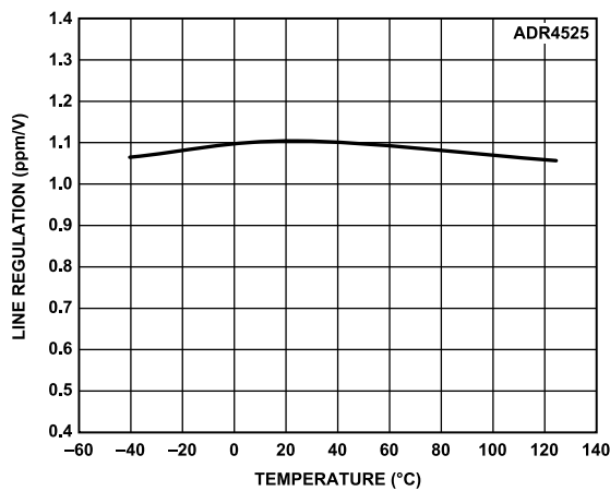
Figure 25. ADR4525 Line Regulation vs. Temperature
