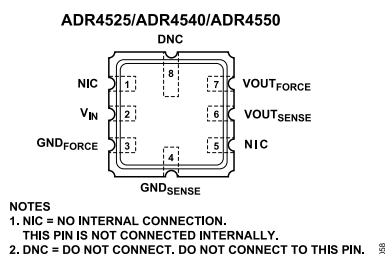
Figure 4. 8-Lead LCC Pin Configuration
