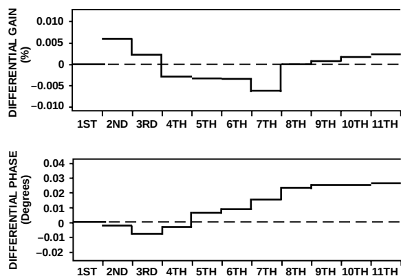
Figure 23. Differential Gain and Phase Error, G = 2 , NTSC Input Signal, R_L = 150\text{ }\Omega , V_S = 5\text{ V}
