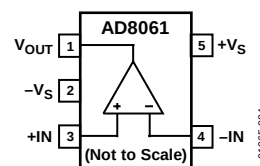
Figure 4. 5-Lead SOT-23 (RJ)
