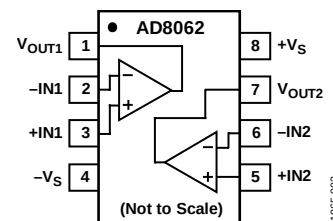
Figure 2. 8-Lead SOIC (R)/MSOP (RM)
