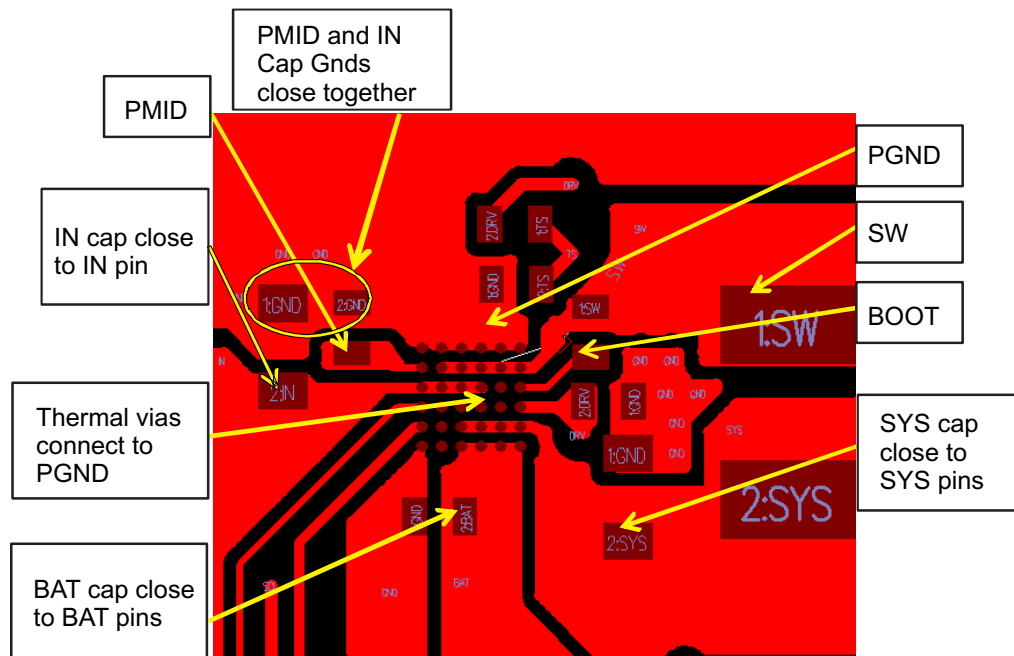
Figure 43. Recommended bq2426x PCB Layout for WCSP Package
