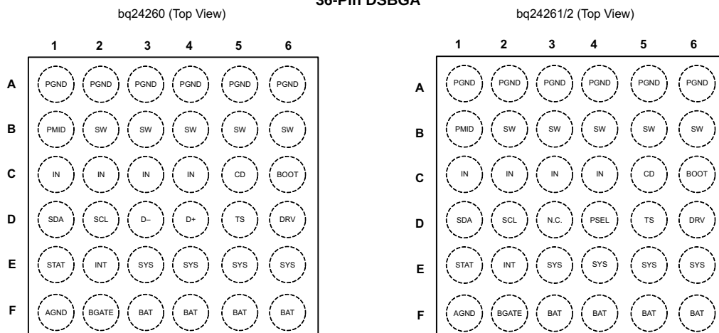
YFF Package 36-Pin DSBGA
