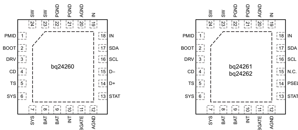
RGE Package 24-Pin VQFN (Top View)
