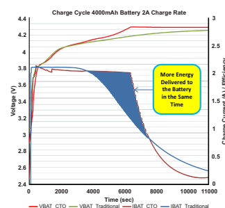
Charge Time Optimizer Effect
