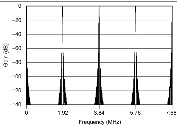
Figure 33. Frequency Response Out to 7.68 MHz for Data Rate = 30 kSPS
