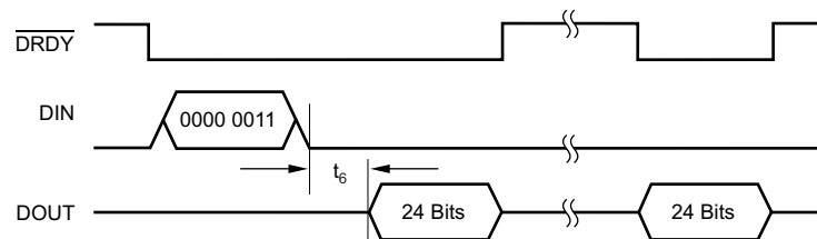
Figure 42. RDATA Command Sequence
