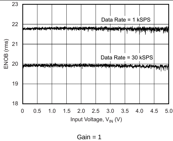
Figure 17. Effective Number of Bits vs Input Voltage
