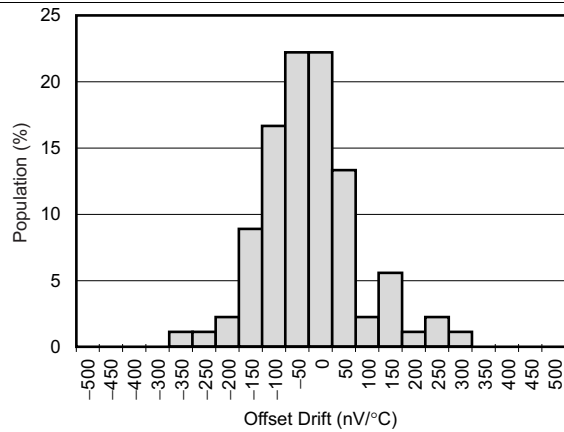
Figure 5. Offset Drift Histogram
