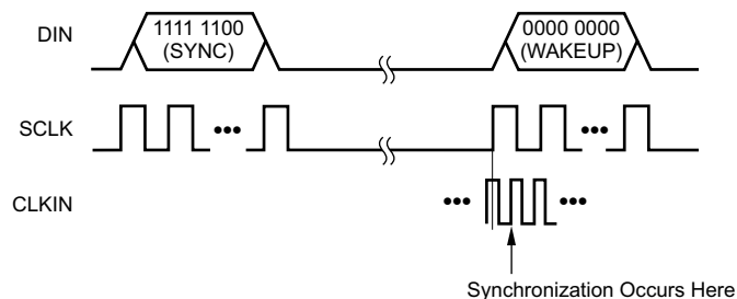
Figure 48. SYNC Command Sequence
