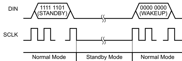
Figure 47. STANDBY Command Sequence
