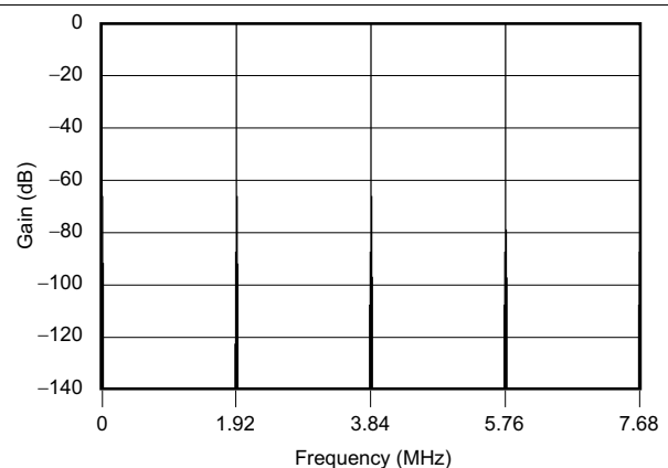
Figure 34. Frequency Response Out to 7.68 MHz for Data Rate = 2.5 SPS
