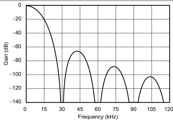
Figure 31. Frequency Response for Data Rate = 30 kSPS
