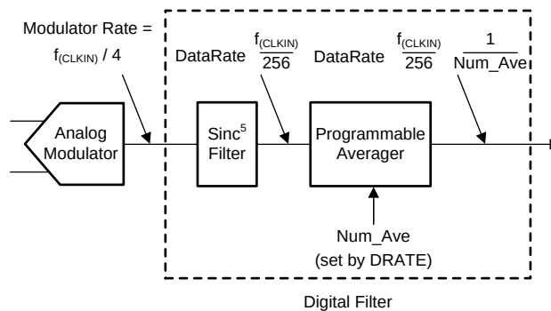
Figure 30. Block Diagram of the Analog Modulator and Digital Filter
