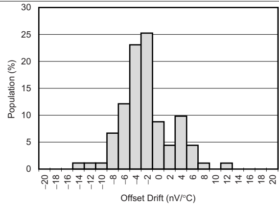
Figure 6. Offset Drift Histogram
