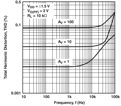
Figure 32. Total Harmonic Distortion vs Frequency, V_{DD} = \pm 1.5 V
