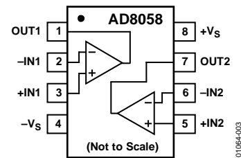
Figure 3. RM-8 (MSOP) and R-8 (SOIC)
