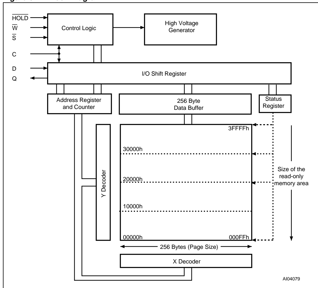
Figure 6. Block Diagram
