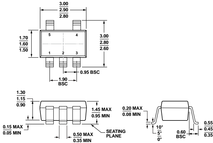
COMPLIANT TO JEDEC STANDARDS MO-178-AA Figure 51. 5-Lead Small Outline Transistor Package [SOT-23] (RJ-5) Dimensions shown in millimeters
