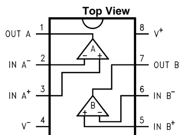
Figure 3. 8-Pin VSSOP Package See Package Number DGK0008A
