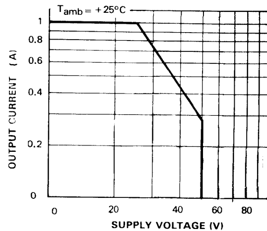
Figure 8: Safe Operating Area (non repetitive surge)
