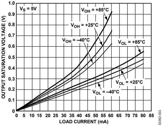
Figure 31. AD8051/AD8052 Output Saturation Voltage vs. Load Current
