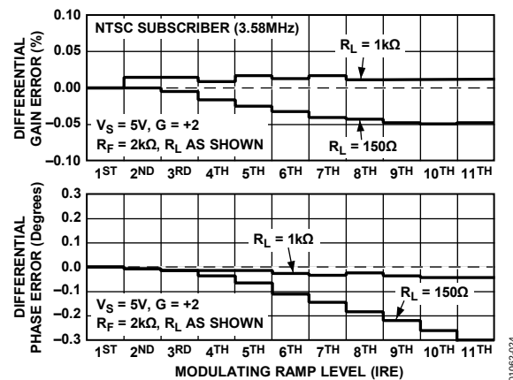
Figure 24. AD8054 Differential Gain and Phase Errors
