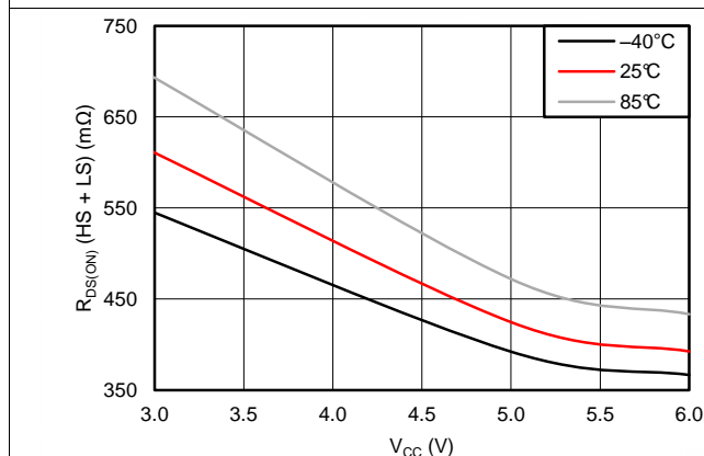
Figure 5. R_{DS(ON)} HS + LS vs V_{VCC}
