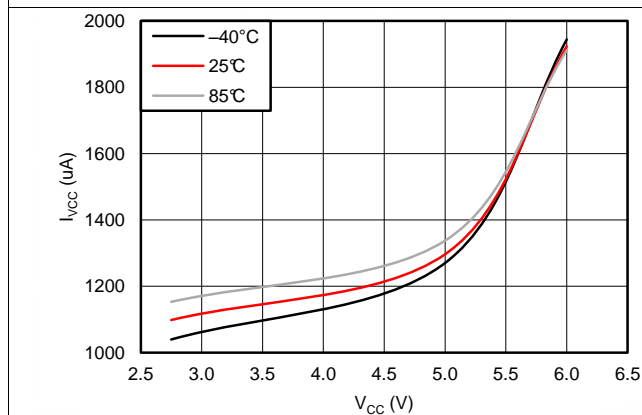
Figure 3. I_{VCC} vs V_{VCC}
