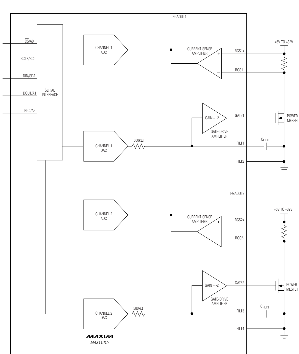
Figure 6. MAX11015 Class AB Analog Control
