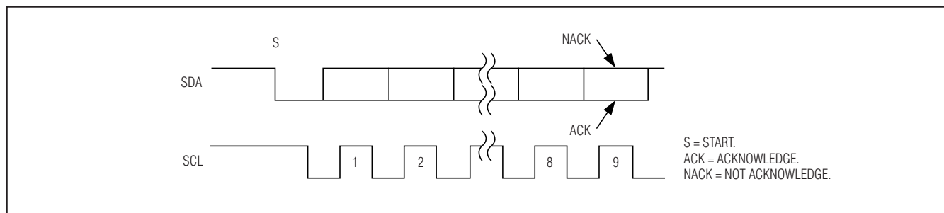
Figure 12. Acknowledge Bits
