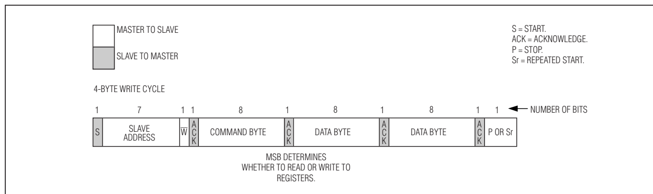
Figure 15. Write Cycle
