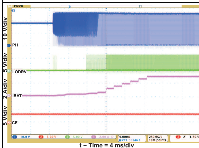
Figure 3. Current Soft-Start (CE = 1)
