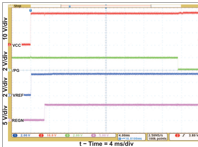
Figure 1. REF, REGN, and \overline{\text{PG}} Power Up (CE = 1)
