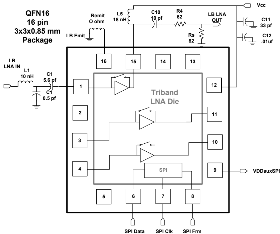
Figure 4. 880 MHz LNA Application Schematic
