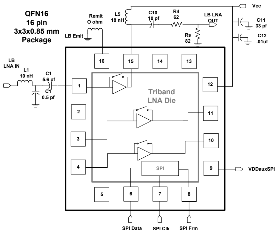
Figure 5. 950 MHz LNA Application Schematic
