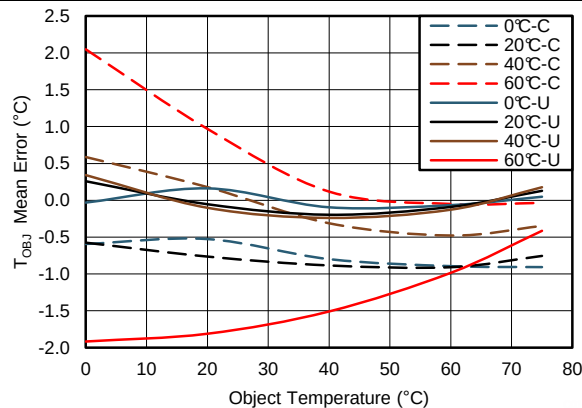
Figure 20. Mean Calibration Error, Wide Range Over T_{DIE}
