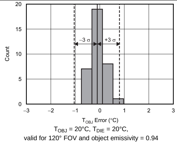
Figure 2. Typical Object Temperature Error
