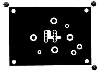
FIGURE 1C. BOTTOM LAYOUT
