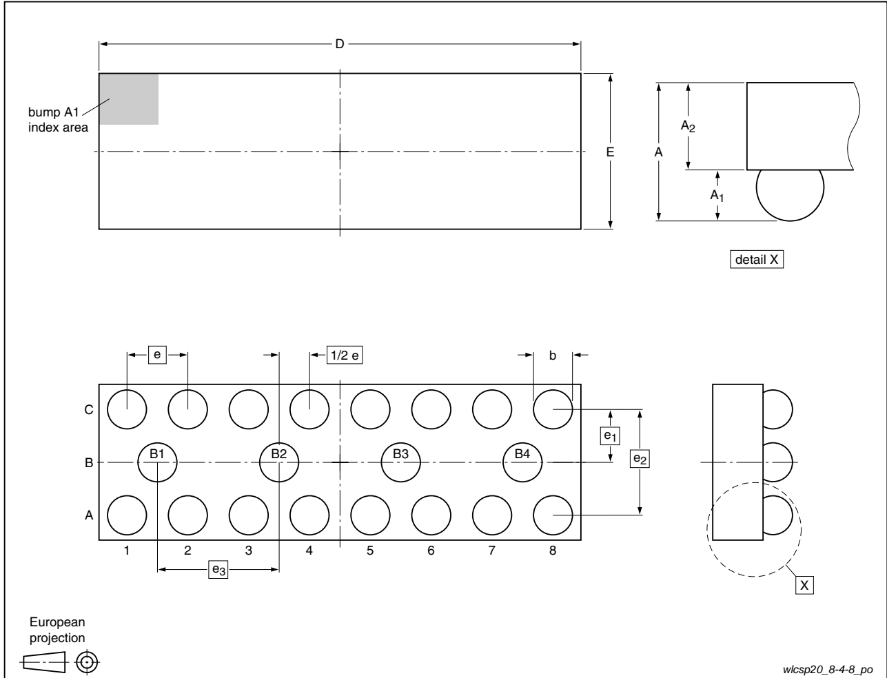
Fig 8. Package outline IP3088CX20 (WLCSP20)
