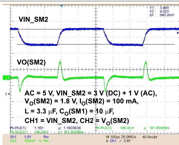
Figure 52. Line Transient
