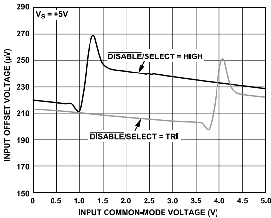
Figure 45. Input Offset Voltage vs. Input Common-Mode Voltage, V_S = 5\text{ V}
