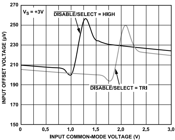
Figure 46. Input Offset Voltage vs. Input Common-Mode Voltage, V_S = 3\text{ V}
