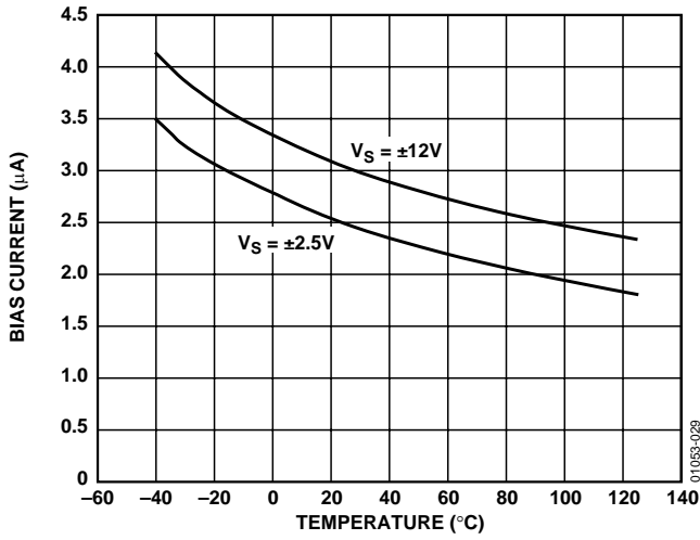
Figure 29. Bias Current vs. Temperature
