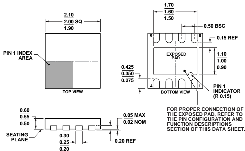
Figure 34. 8-Lead Lead Frame Chip Scale Package [LFCSP_UD] 2.00 x 2.00 mm Body, Ultra Thin, Dual Lead (CP-8-10)
