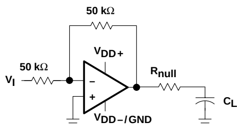
Figure 62. Series-Resistance Circuit
