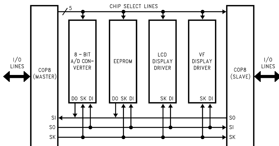
Figure 5-23. MICROWIRE/PLUS Application
